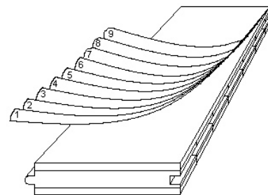
1) Primer Coat 2) Fill Coat w/aluminum oxide & ceramic particles 4, 5, 6) Fill Coats 7, 8, 9) Anti-Scratch Top Coats
